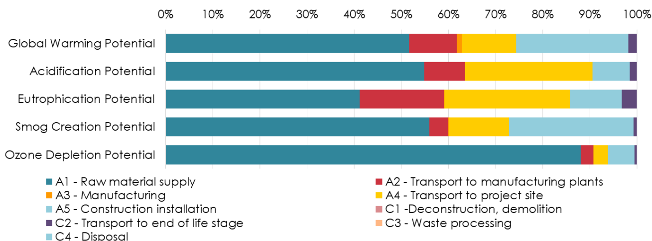
Figure 3: Relative contributions of the main processes in the production of MM6125®EU
