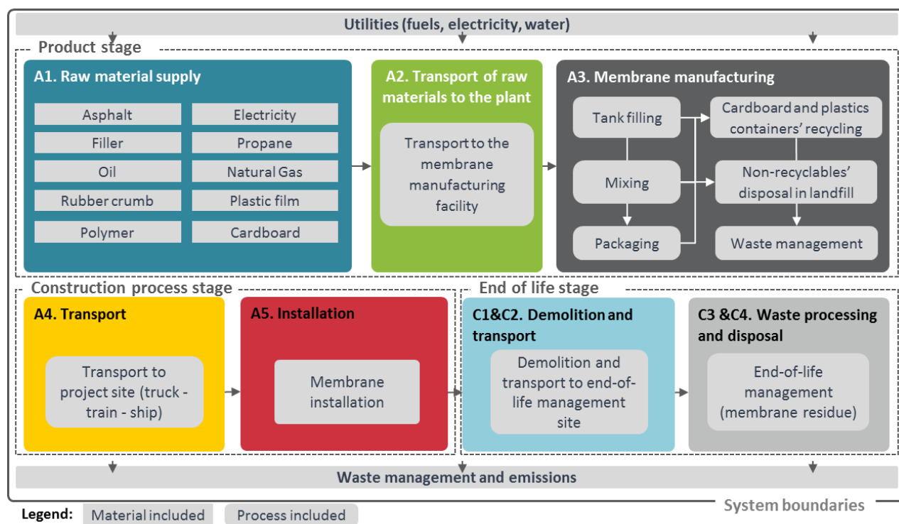
Figure 2: Process flow for the life cycle of Monolithic Membrane 6125®EU
