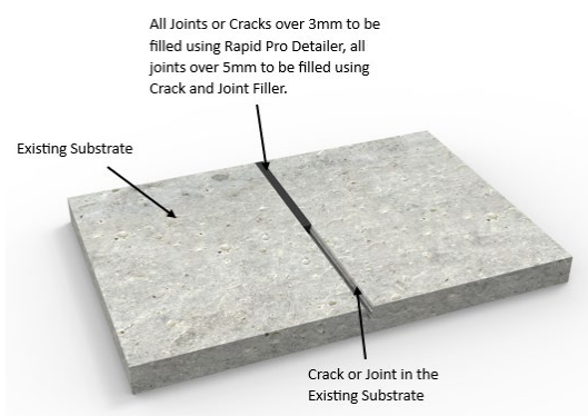
Diagram 2 - Detailing cracks and joints
