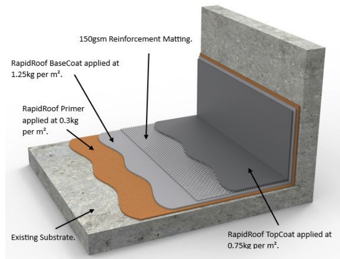
Diagram 3 - Detailing angles
